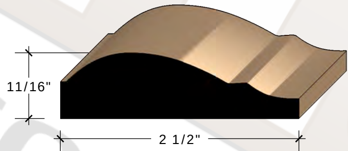
11/16" X 2 1/2" SF-1 CASING FINGERJOINT PINE
