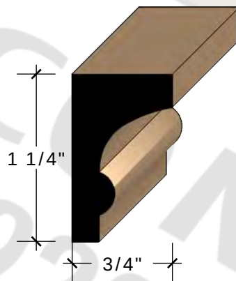
3/4" X 1 1/4" MANTLE MOULD POPLAR More info
