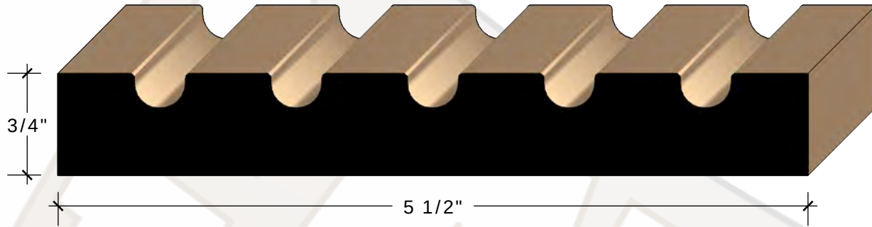
3/4" X 5 1/2" FLUTED POPLAR More info
