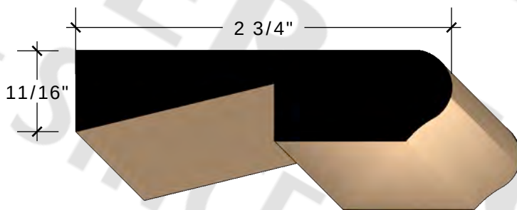
11/16" X 2 3/4" RABBETED STOOL FINGERJOINT PINE CLEAR FIR More info
