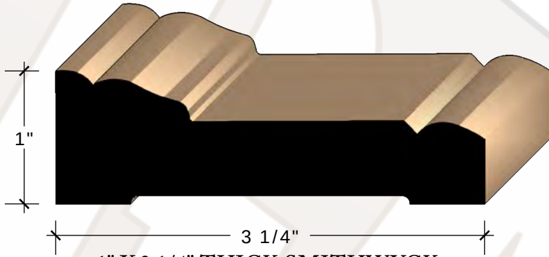
1" X 3 1/4" THICK SMITHWYCK SP-376 CASING FINGERJOINT PINE
