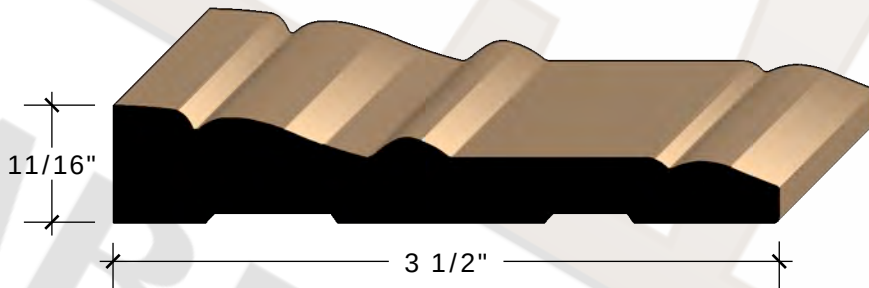
11/16" X 3 1/2" LC-11 CASING FINGERJOINT PINE
