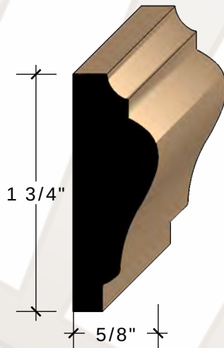
5/8" X 1 3/4" G-37 PANEL MOULD POPLAR More info
