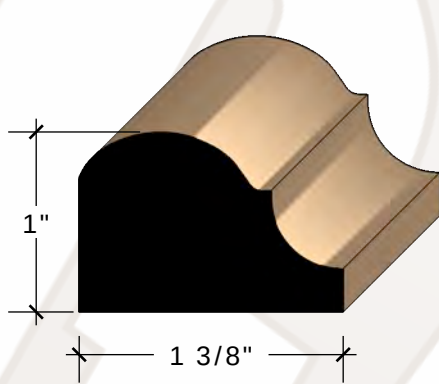
1" X 1 3/8" SHELF EDGE POPLAR More info
