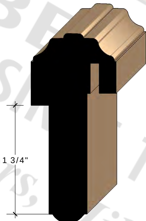
1" X 2" BEADED BRICK MOULD FINGERJOINT PINE More info
