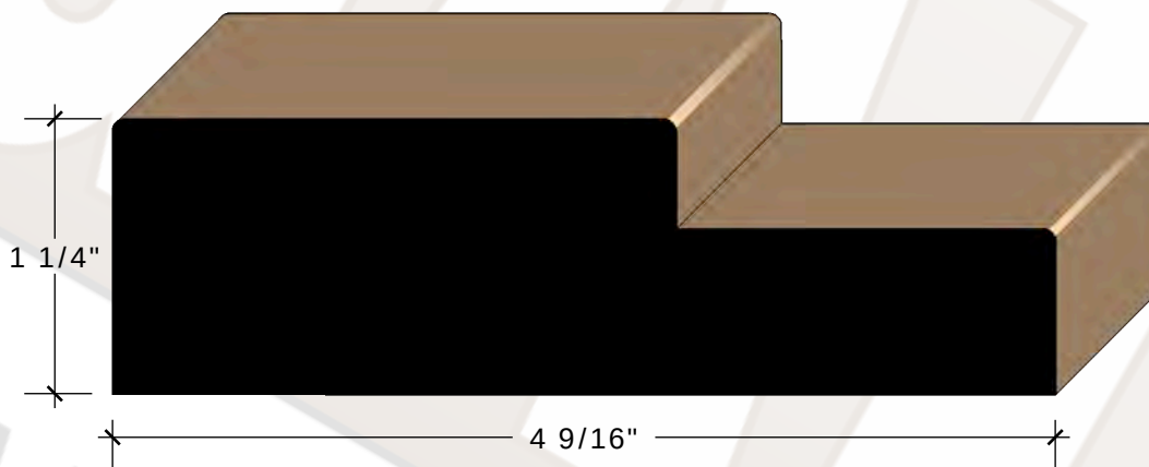
1 1/4" X 4 9/16" OUTSIDE JAMB FINGER JOINT PINE More info
