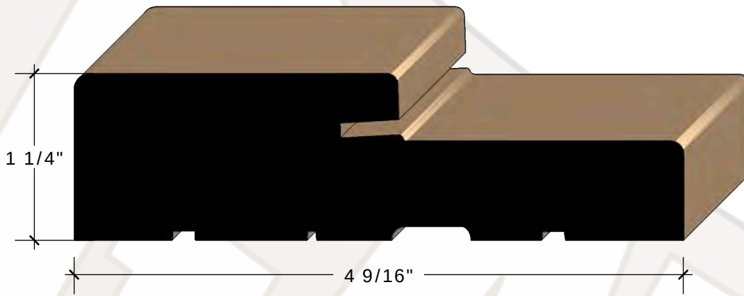
1 1/4" X 4 9/16" METAL DOOR JAMB FINGER JOINT PINE More info
