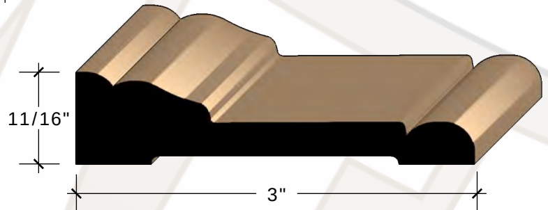
11/16" X 3" SMITHWYCK CASING FINGERJOINT PINE
