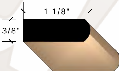
3/8" X 1 1/8" NOSING CLEAR FIR More info
