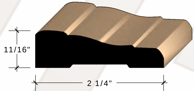
11/16" X 2 1/4" M/E CASING FINGERJOINT PINE More info
