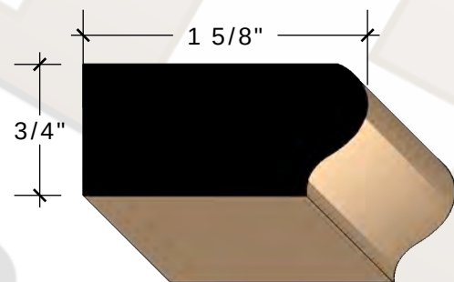
3/4" X 1 5/8" NOSING FINGERJOINT PINE More info
