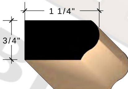
3/4" x 1 1/4" NOSING POPLAR/CLEAR FIR More info
