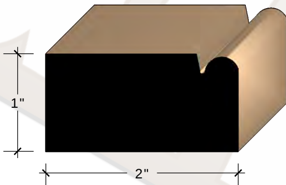
1" X 2" BEADED BRICK MOULD FINGERJOINT PINE More info
