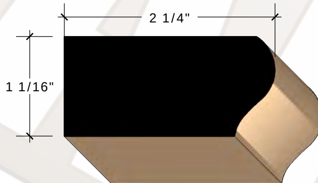
1 1/16" X 2 1/4" RB NOSING FINGERJOINT PINE More info
