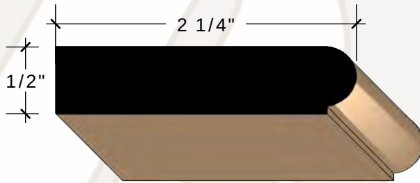
1/2" X 2 1/4" SCRIBE POPLAR More info
