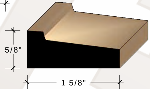
11/16" X 1 5/8" DRIP CAP CLEAR FIR More info
