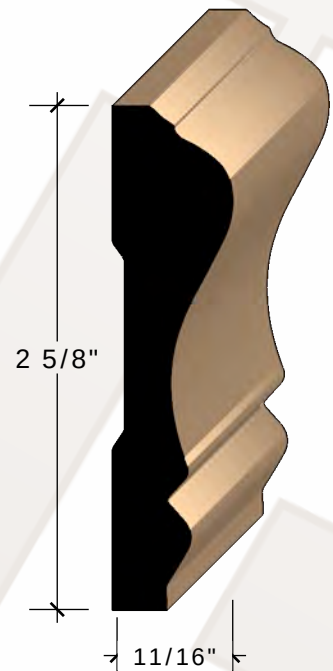
11/16" X 2 5/8" CHAIRRAIL FINGERJOINT PINE More info
