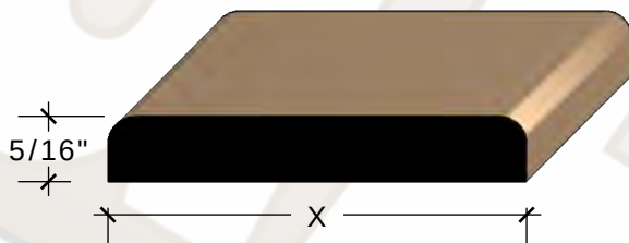
5/16" X MULL STOCK AVAILABLE IN WIDTHS UP TO 11 1/4" POPLAR More info
