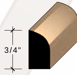
7/16" X 3/4" SHOE MOULD FINGERJOINT PINE CLEAR FIR RED/WHITE OAK More info
