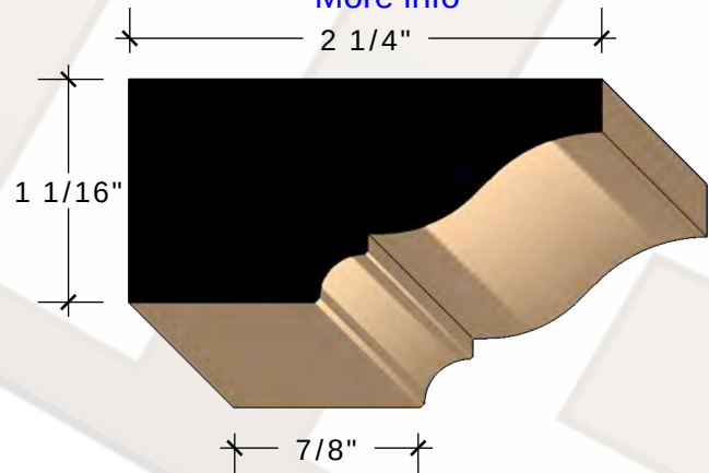
1 1/16" X 2" CABINET HEAD POPLAR More info
