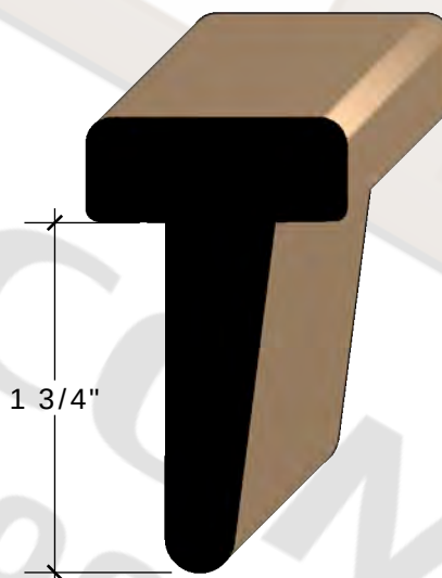
ROUND EDGE T-ASTRIGAL FOR 1 3/4" & 1 3/8" DOORS CLEAR FIR More info
