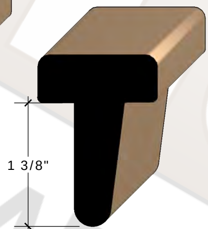
ROUND EDGE T-ASTRIGAL FOR 1 3/4" & 1 3/8" DOORS CLEAR FIR More info
