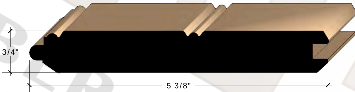
1 X 6 CLEAR YELLOW PINE T&G BEADED W/V-JOINT BACKSIDE More info
