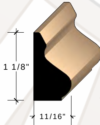
11/16" X 1 1/8" BASE CAP FINGERJOINT PINE/ CLEAR FIR More info
