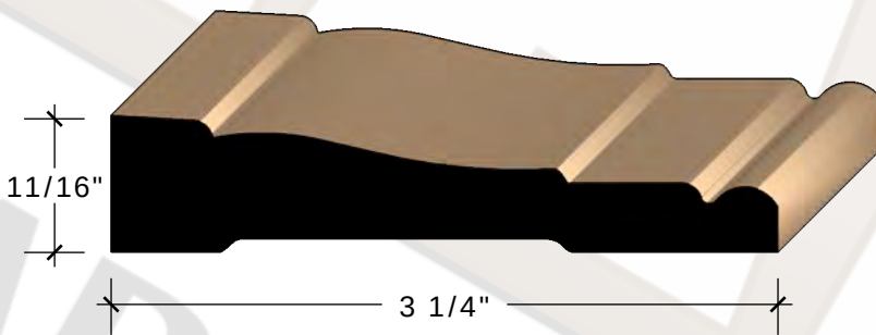
11/16" X 3 1/4" BEADED CASING FINGERJOINT PINE More info
