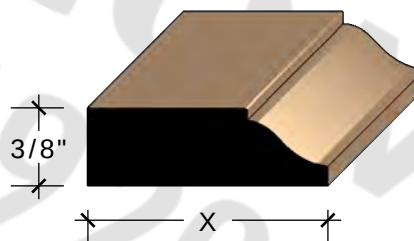
3/8" PG STOP 9/16" TO 2" IN WIDTH FINGERJOINT PINE CLEAR FIR More info
