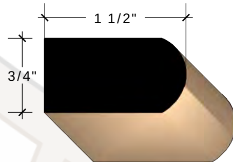
3/4" X 1 1/2" AY-70 BULL NOSING POPLAR More info
