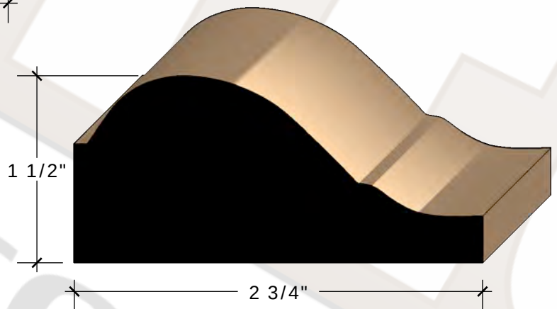
1 1/2" X 2 3/4" FOG-1 CASING FINGERJOINT PINE
