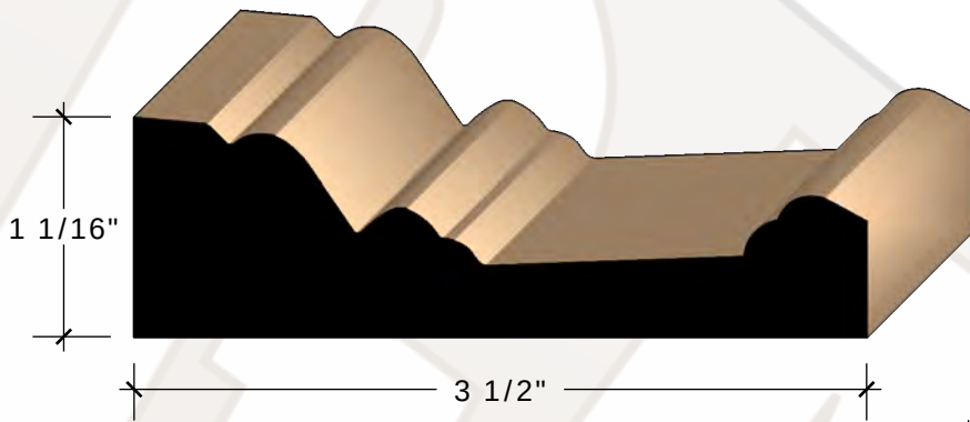
1 1/16" X 3 1/2" HOWE CASING FINGERJOINT PINE
