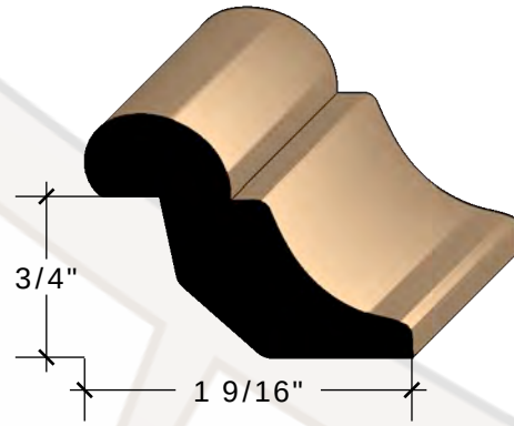
11/16" X 1 7/8" DROP MOULD FINGERJOINT More info
