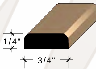
1/4" X 3/4" SCREEN MOULD CLEAR FIR More info
