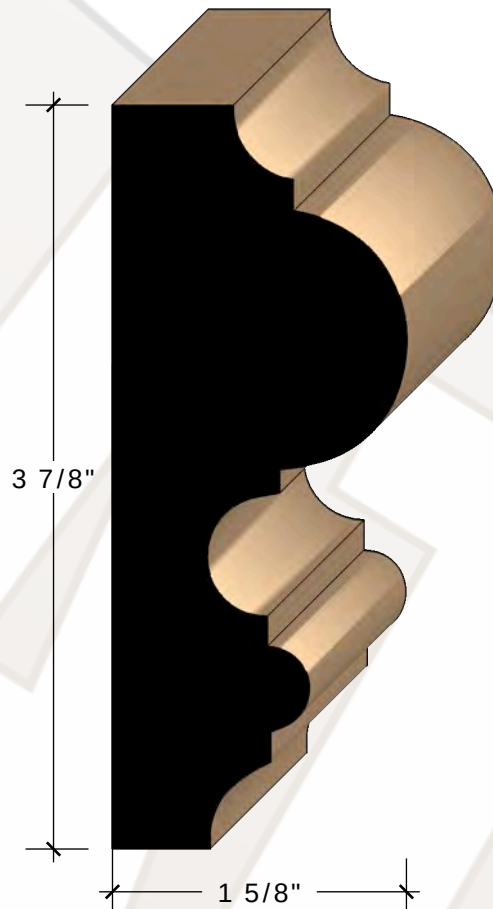
1 5/8" X 3 7/8" FIREPLACE MOULD POPLAR More info
