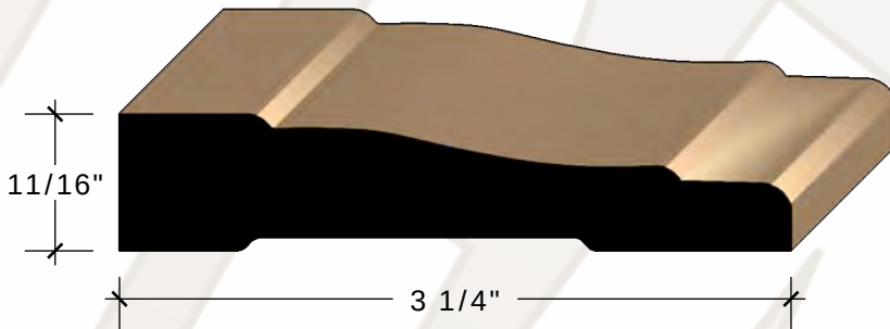
11/16" X 3 1/4" M/E CASING FINGERJOINT PINE/ CLEAR FIR More info
