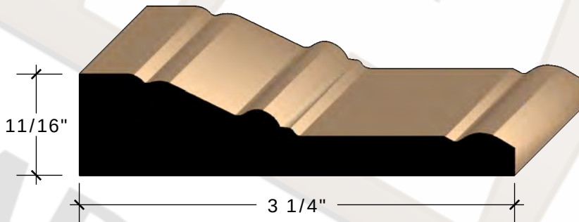
11/16" X 3 1/4" GRANT CASING FINGERJOINT PINE
