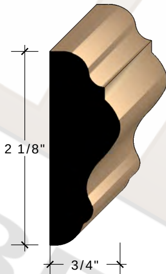
3/4" X 2 1/8" CP-1 PANEL MOULD FINGERJOINT PINE More info
