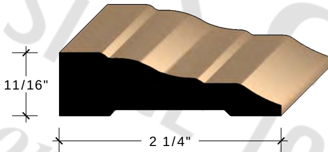
11/16" X 2 1/4" 366 CASING FINGERJOINT PINE More info
