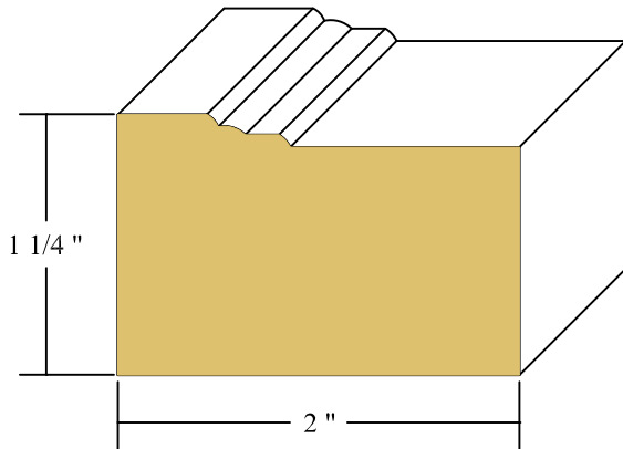
1 1/4" X 2" ROW BRICKED MOULD FINGERJOINT PINE/PVC
