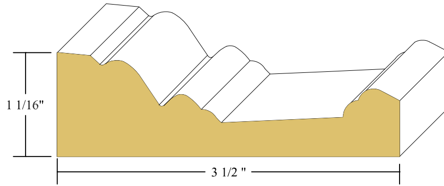
1 1/16" X 3 1/2" HOWE CASING FINGERJOINT PINE
