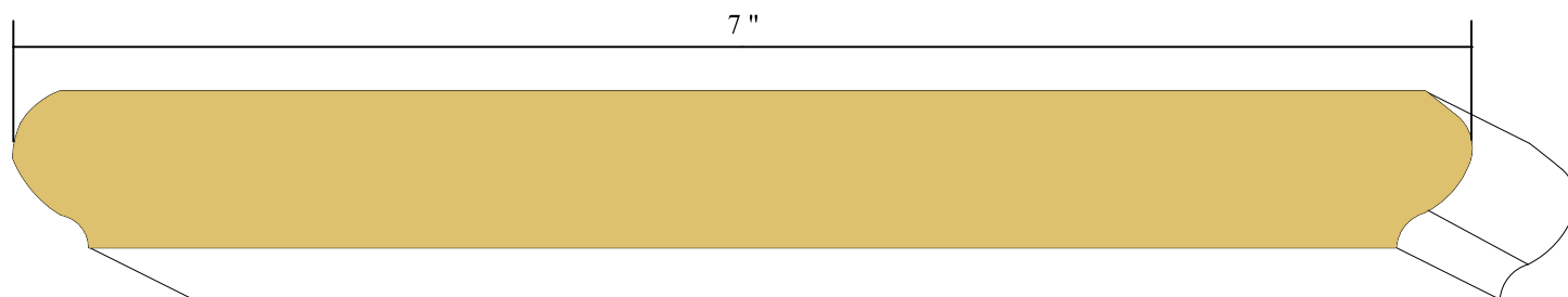
3/4" X 7" NOSE 4 (LOW WALL CAP) POPLAR
