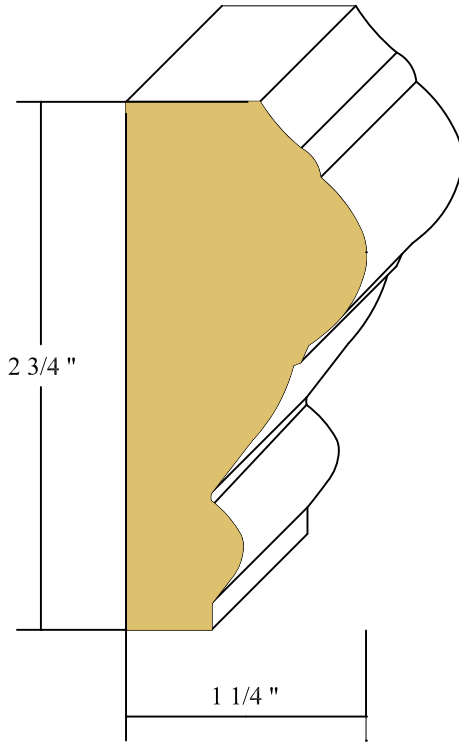
1 1/4" X 2 5/8" BD-1 CHAIRRAIL CLEAR POPLAR
