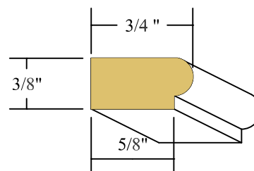
3/8" X 3/4" QUIRK BEAD POPLAR
