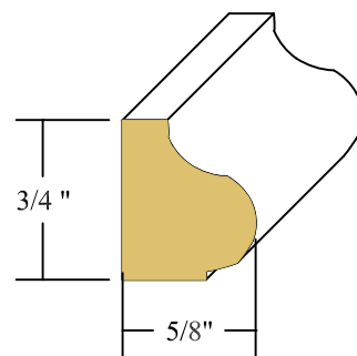
5/8" X 3/4" BASE CAP CLEAR
