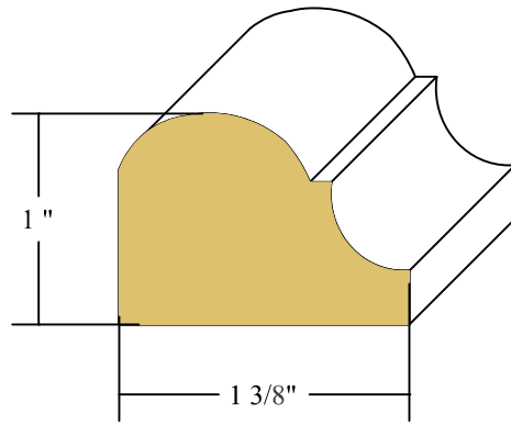
1" X 1 3/8" SHELF EDGE POPLAR
