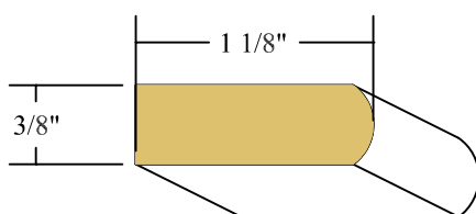
3/8" X 1 1/8" NOSING CLEAR FIR
