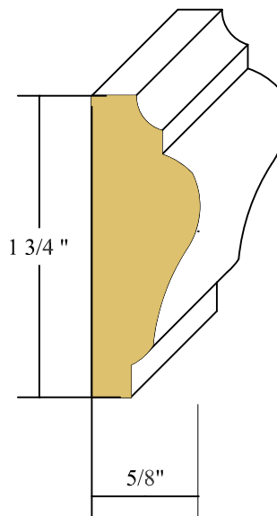
5/8" X 1 3/4" G-37 PANEL MOULD POPLAR
