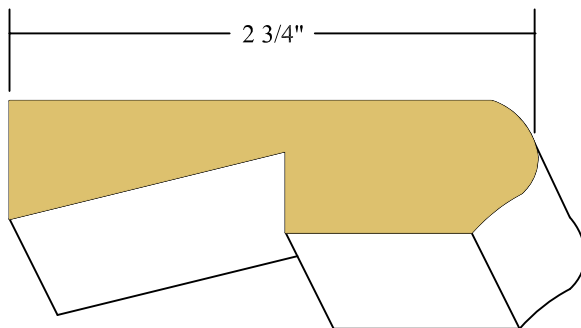
11/16" X 2 3/4" RABBETED STOOL FINGERJOINT PINE
