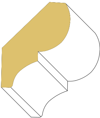
5/8" X 1 3/4" BED MOULD CLEAR FIR
