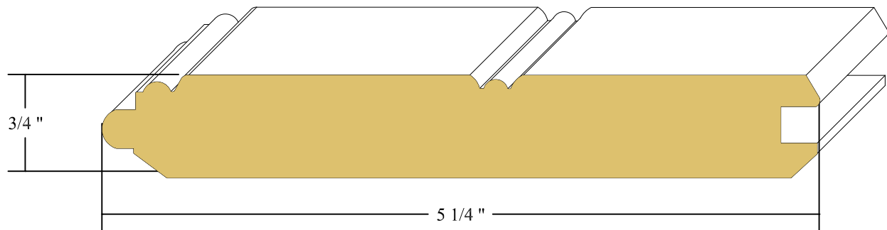
1" X 6" CLEAR YELLOW PINE T&G BEADED W/V-JOINT BACKSIDE
