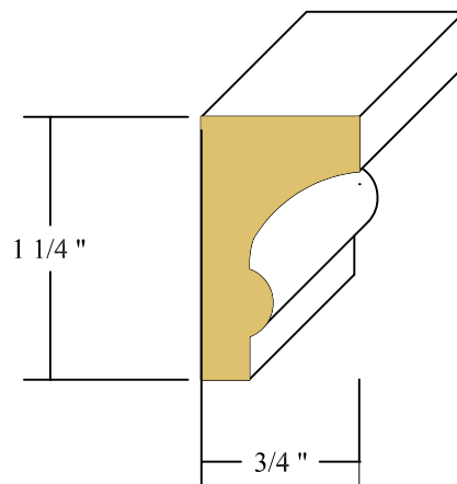
3/4" x 1 1/4" MANTLE MOULD POPLAR
