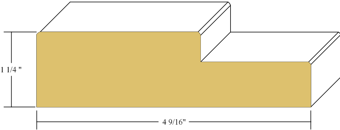
1 1/4" X 4 9/16" OUTSIDE JAMB FINGER JOINT PINE
