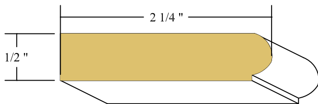
1/2" X 2 1/4" SCRIBE POPLAR
