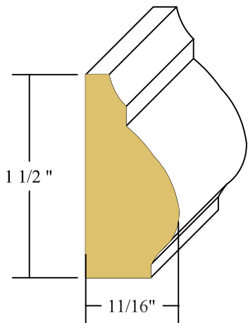
11/16" x 1 1/2" THUMBNAIL BASE CAP FINGER JOINT PINE
