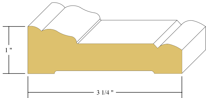
1" X 3 1/4" THICK SMITHWYCK SP-376 CASING FINGERJOINT PINE
