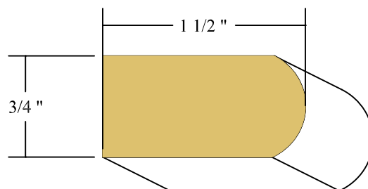
3/4" X 1 1/2" AY-70 BULL NOSING POPLAR
