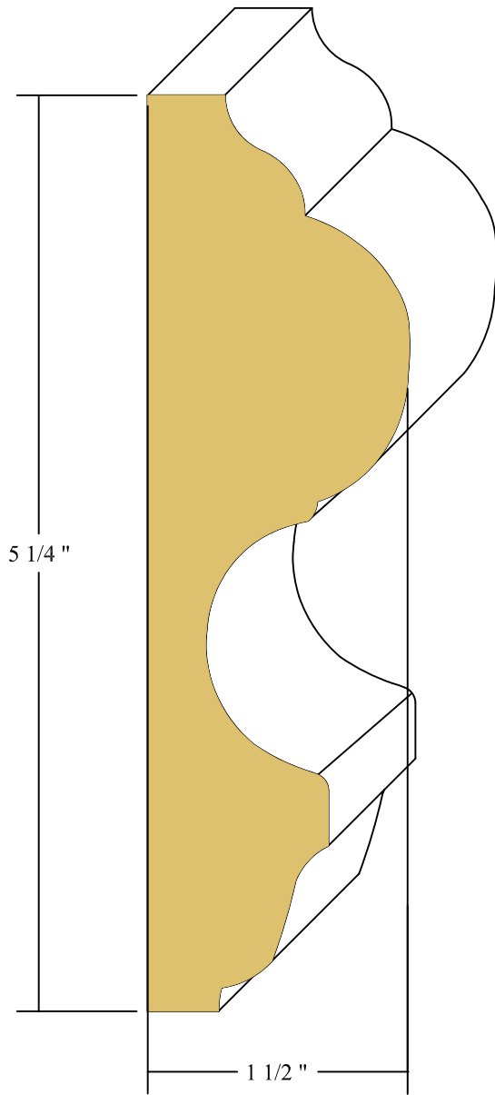
1 1/2" X 5 1/4" WIDE FIREPLACE MOULD POPLAR
