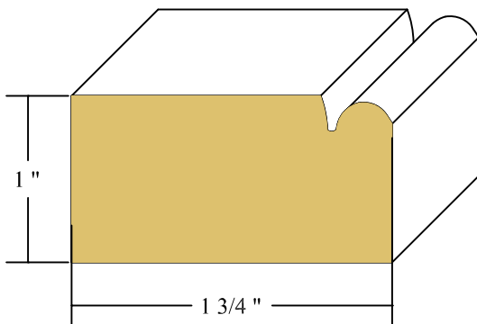
1" X 2" BEADED BRICK MOULD FINGER JOINT PINE
