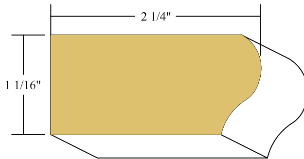
1 1/16" X 2 1/4" RB NOSING CLEAR POPLAR
