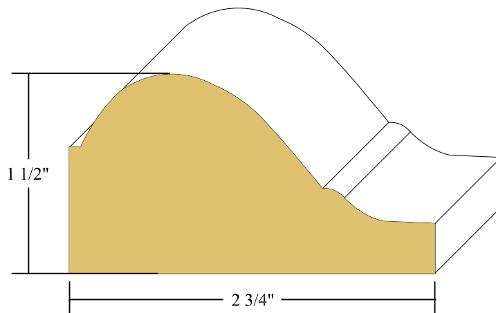
1 1/2" X 2 3/4" FOG-1 CASING POPLAR
