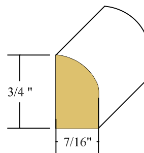
7/16" X 3/4" SHOE MOULD FINGERJOINT PINE PRIMED CLEAR FIR RED/WHITE OAK
