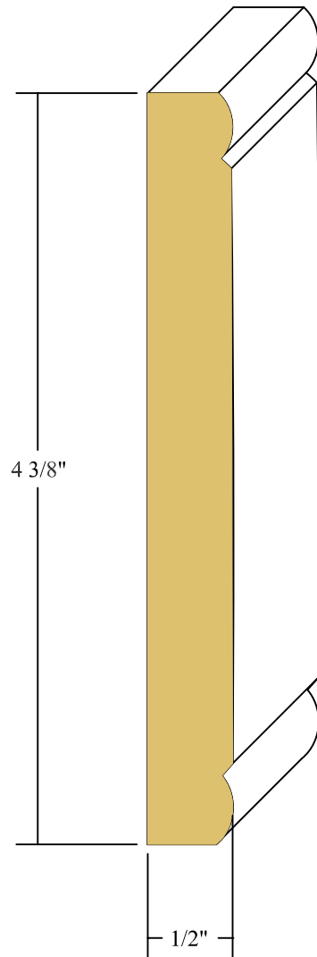
1/2" X 4 3/8" BD-2 CHAIRRAIL FINGERJOINT PINE
