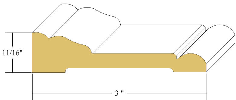
11/16" X 3" SMITHWYCK CASING FINGERJOINT PINE
