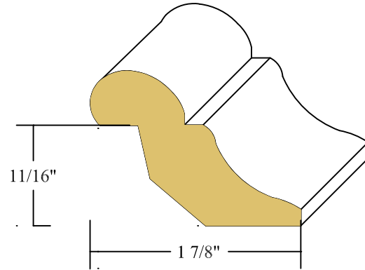
11/16" X 1 7/8" DROP MOULD POPLAR
