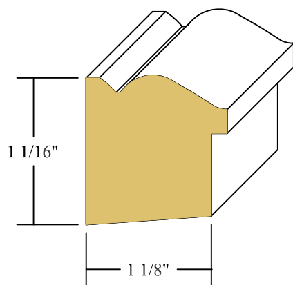
1 1/16" X 1 1/8" BACKBAND FINGERJOINT PINE CLEAR FIR
