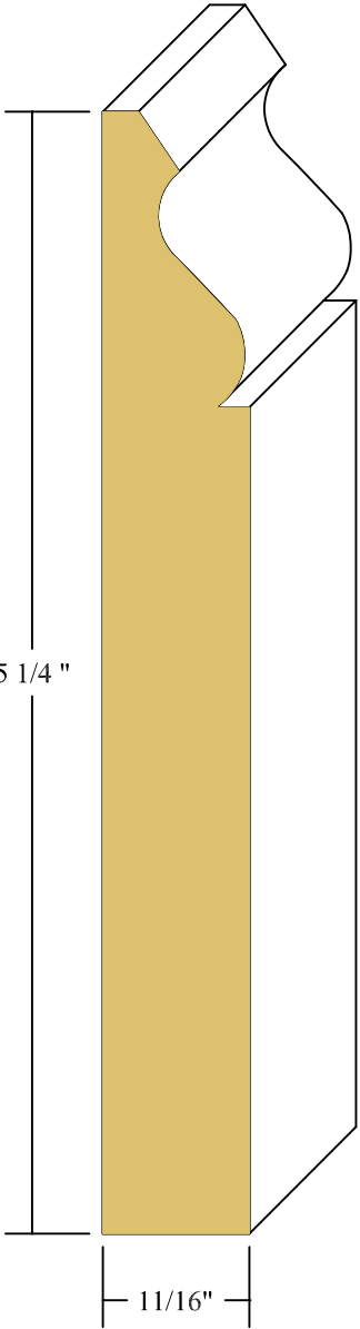
11/16" X 5 1/4" BASE FINGER JOINT PINE/ MDF
