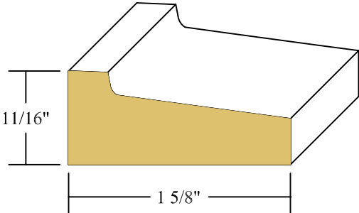
11/16" X 1 5/8" DRIP CAP CLEAR FIR
