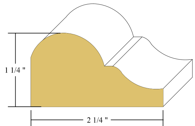
1 1/4" X 2 1/4" JB-1 CASING POPLAR
