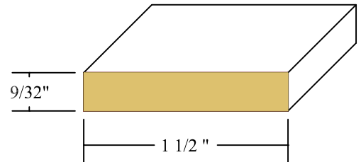
9/32" X 1 1/2" LATTICE CLEAR FIR
