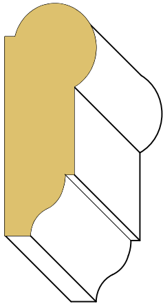
1 1/16" X 1 3/4" PICTURE MOULD FINGER JOINT PINE
