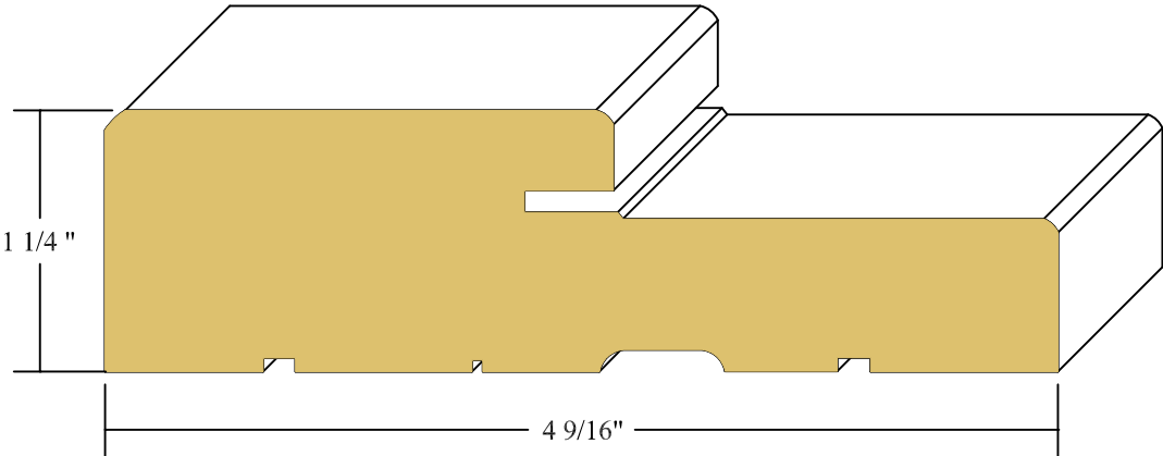
1 1/4" X 4 9/16" METAL DOOR JAMB FINGER JOING PINE
