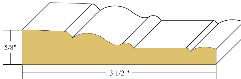
5/8" X 3 1/2" MEMPHIS CASING PRIMED FINGERJOINT
