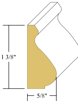
5/8" x 1 3/8" BASECAP CLEAR
