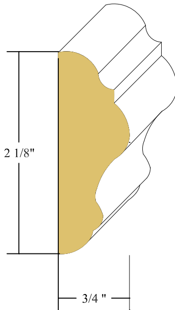
3/4" X 2 1/8" CP-1 PANEL MOULD CLEAR
