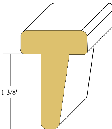
ROUND EDGE T-ASTRIGAL FOR 1 3/4" & 1 3/8" DOORS CLEAR FIR
