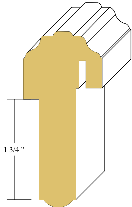
OGEE EDGE T-ASTRIGAL WITH WEATHER STRIPPING PINE/MAHOGANY
